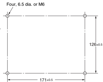
Mounting Hole Dimensions
