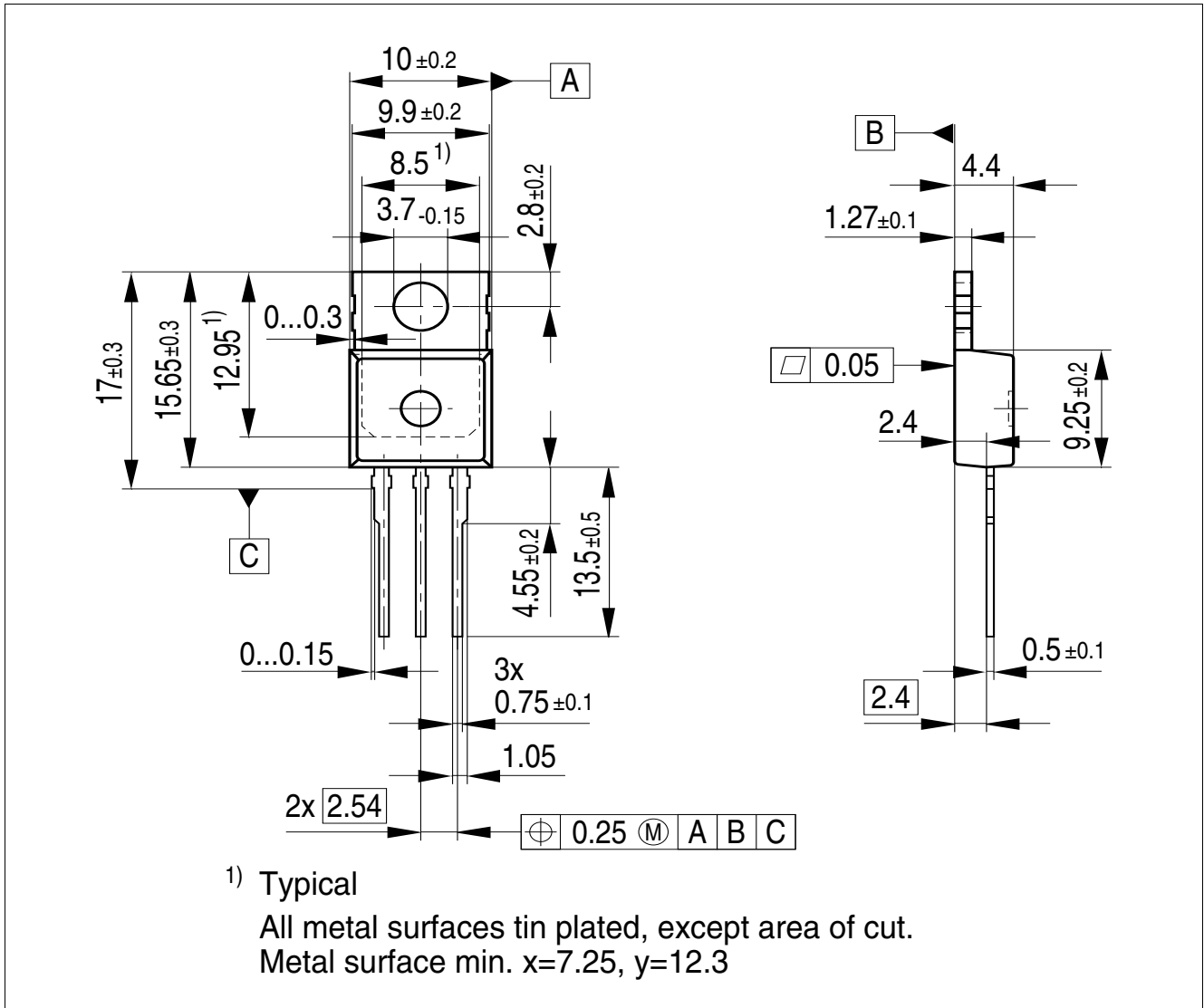
Figure 1 PG-T0220-3-1
