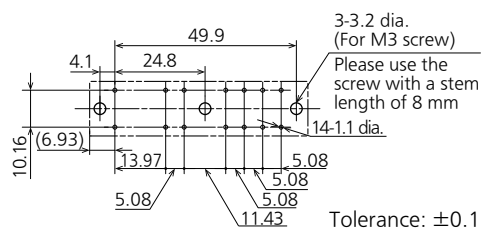
Recommended PC board pattern ( BOTTOM VIEW )
