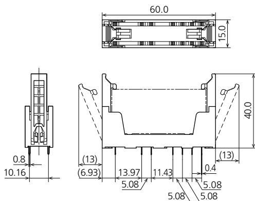
External dimensions
