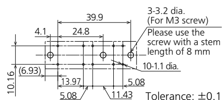
Recommended PC board pattern ( BOTTOM VIEW )
