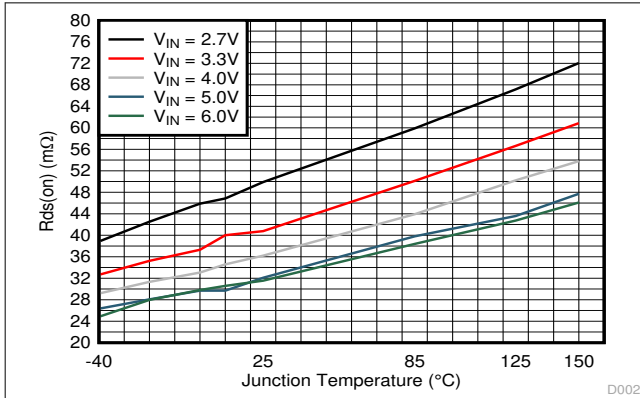
Figure 7-1. R_{ds(on)} of High-side Switch
