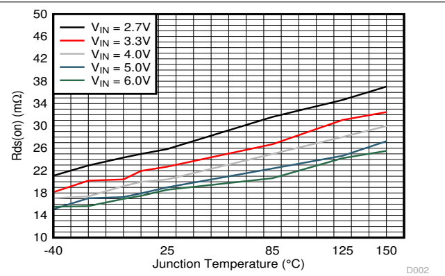
Figure 7-2. R_{ds(on)} of Low-side Switch
