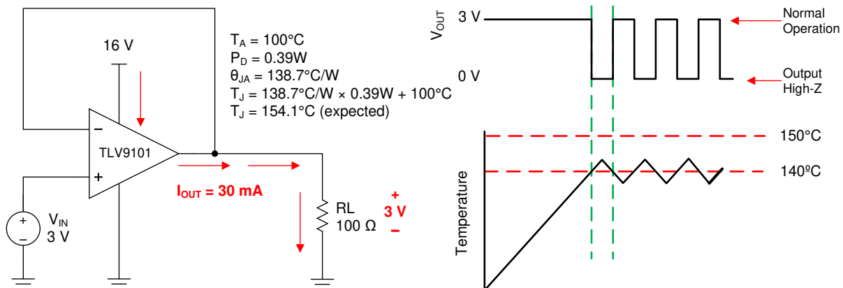
Figure 46. Thermal Protection
