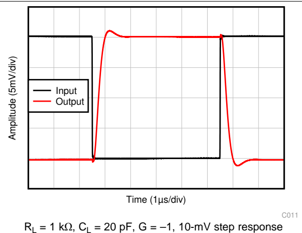
Figure 36. Small-Signal Step Response
