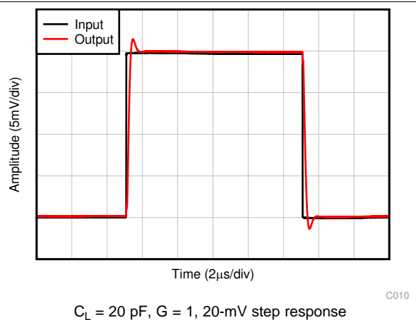
Figure 35. Small-Signal Step Response
