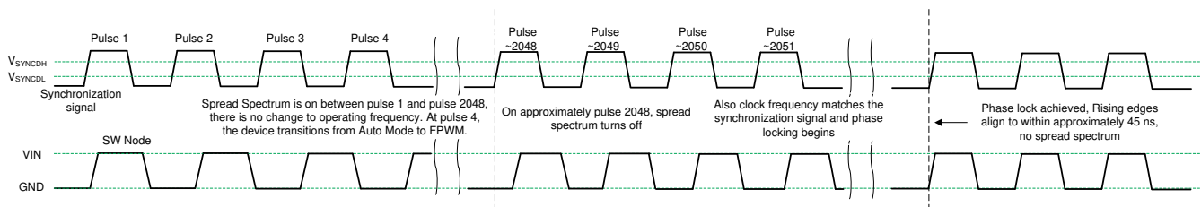
Figure 9-5. Synchronization Process
