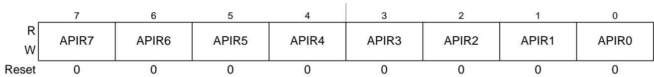
Figure 3-6. Autonomous Periodical Interrupt Rate Low Register (VREGAPIRL)
