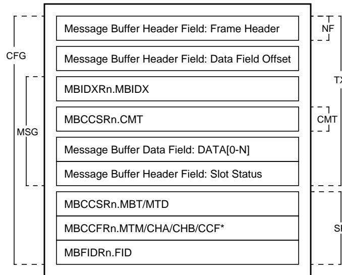
Figure 13-113. Single Transmit Message Buffer Access Regions
