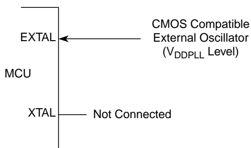
Figure 5-4. External Clock Connections (FSP mode selected)
