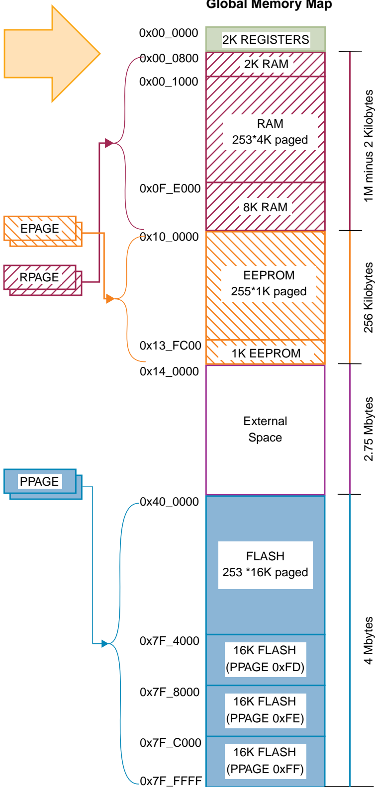
Figure 11-17. Expansion of the Local Address Map
