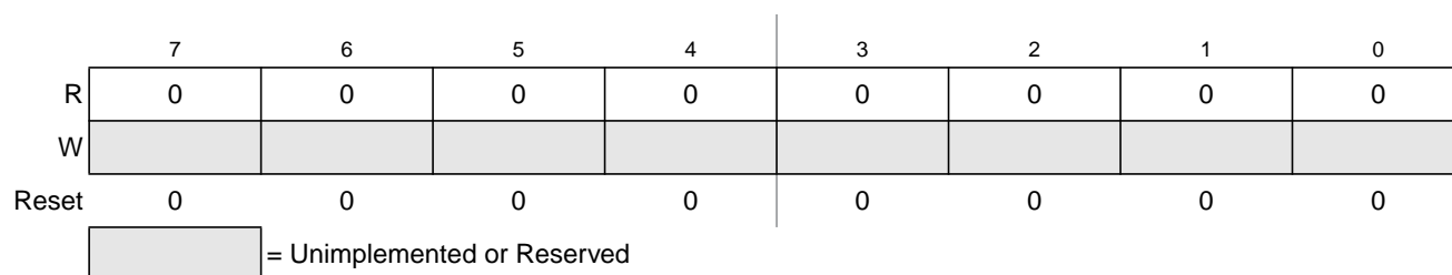
Figure 12-7. Reserved Register (CGMTEST0)
