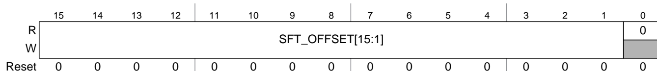
Figure 13-33. Sync Frame Table Offset Register (SFTOR)
