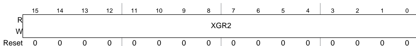
Figure 14-16. XGATE Register 2 (XGR2)
