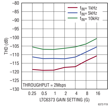
Figure 19. THD for LTC6373 Driving ADAQ4003 (Gain = 1.9)
