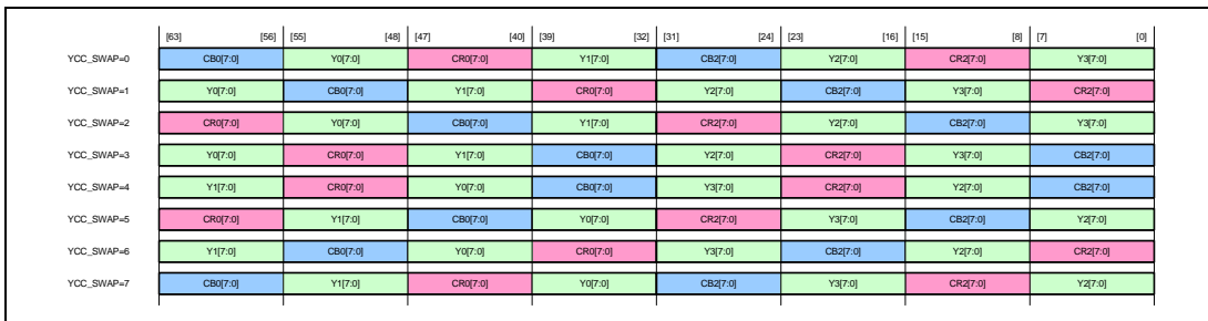
Figure 35.6 YCbCr422 Data Arrangement with Swapping Enabled
