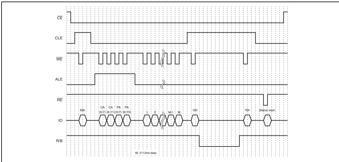
Figure 28.13 Programming Operation Timing for NAND-Type Flash Memory
