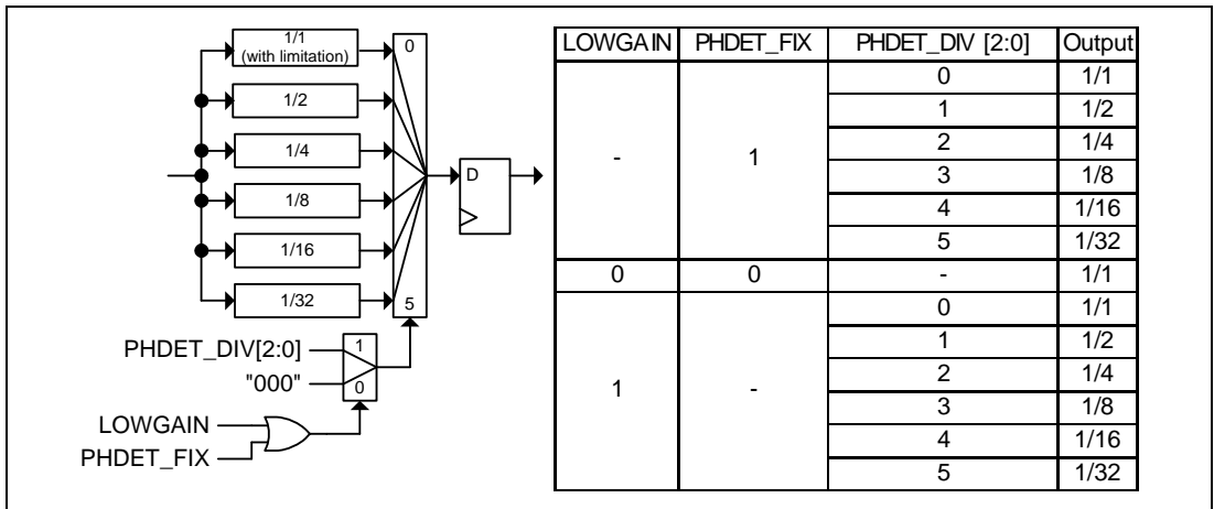
Figure 30.24 Phase Comparator Feedback Adjust
