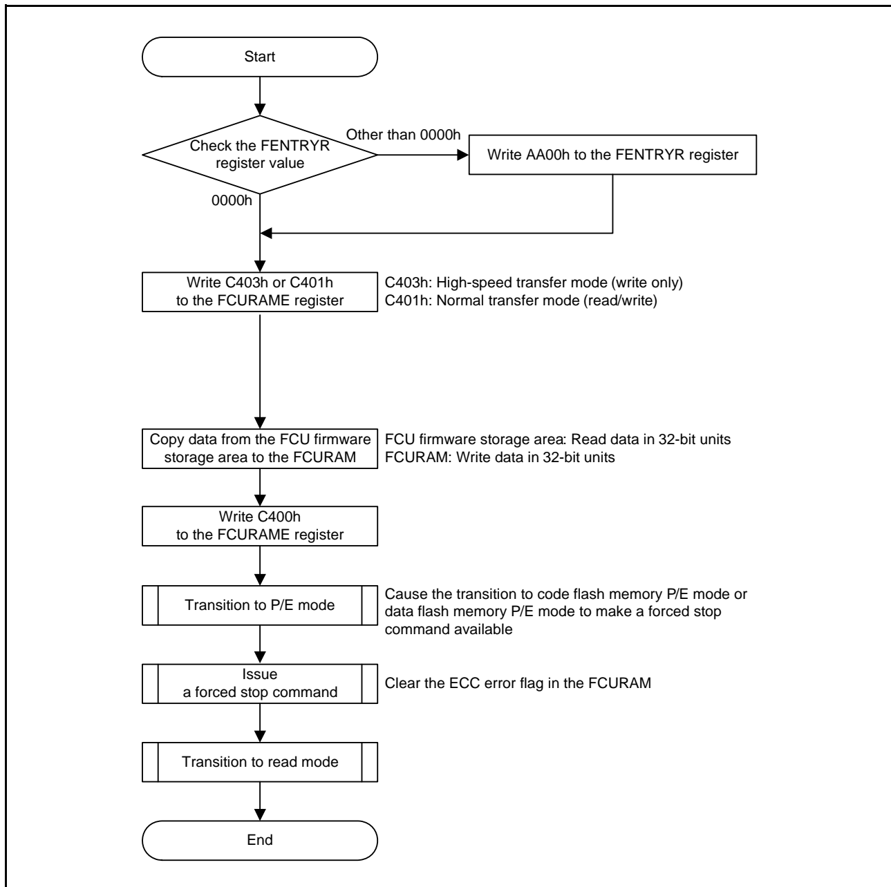
Figure 6.4 Flow for Transferring the FCU Firmware
