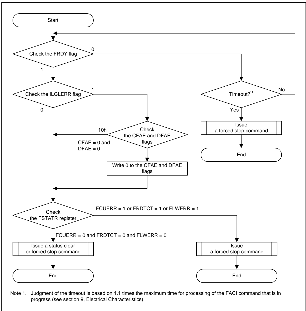
Figure 6.8 Recovery from the Command-Locked State
