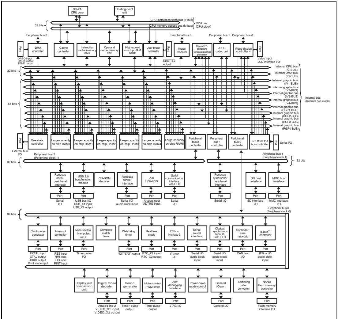
Figure 1.1 Block Diagram
