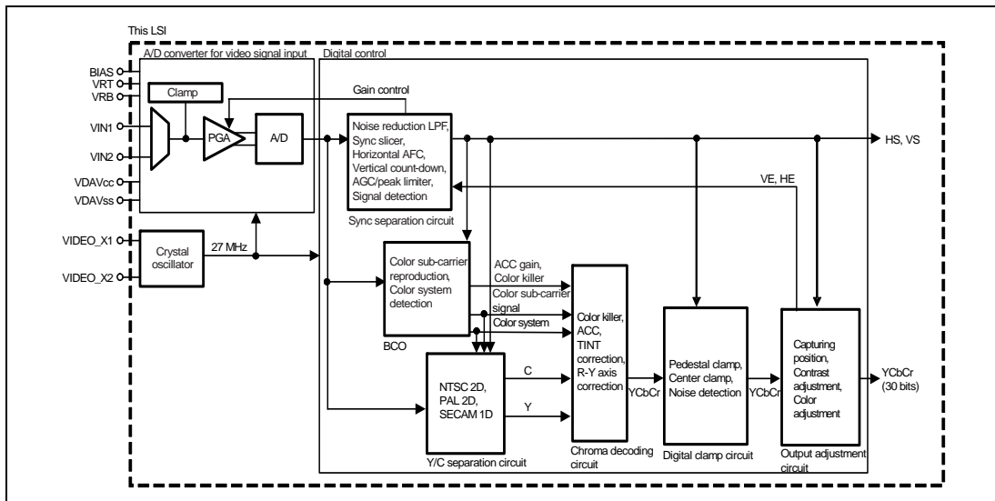
Figure 30.1 Block Diagram
