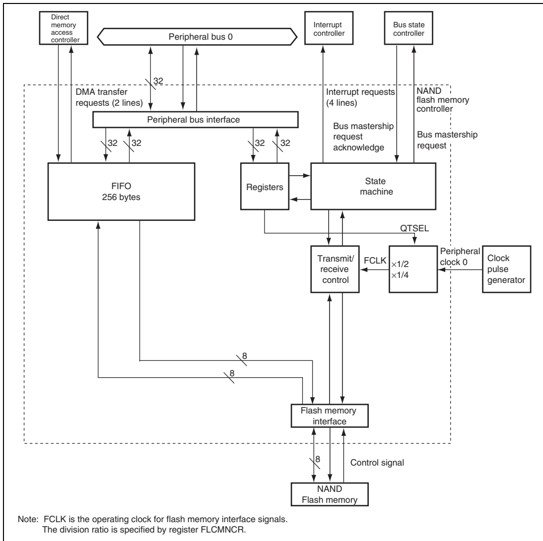
Figure 28.1 Block Diagram
