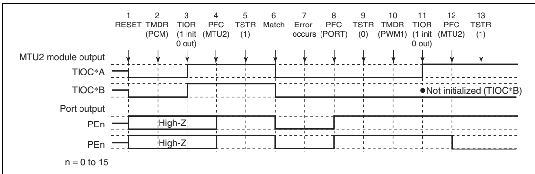
Figure 12.132 Error Occurrence in Phase Counting Mode, Recovery in PWM Mode 1
