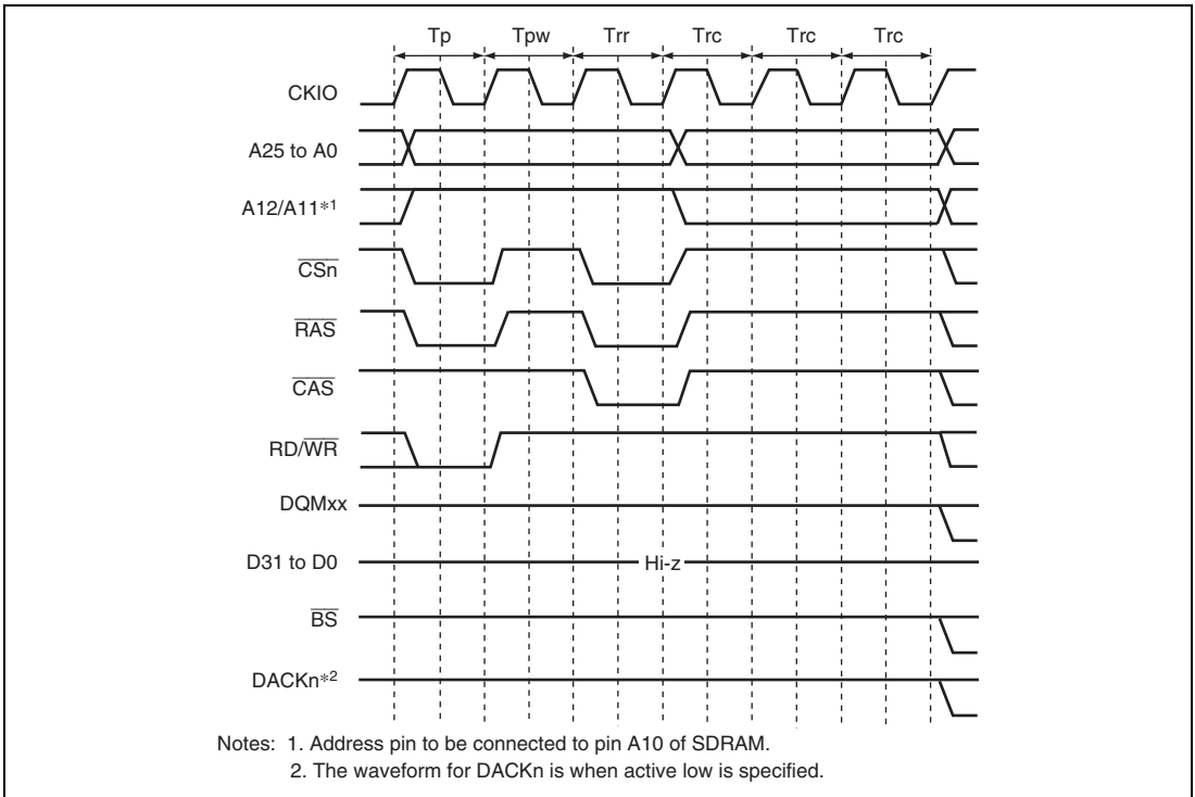
Figure 10.27 Auto-Refresh Timing
