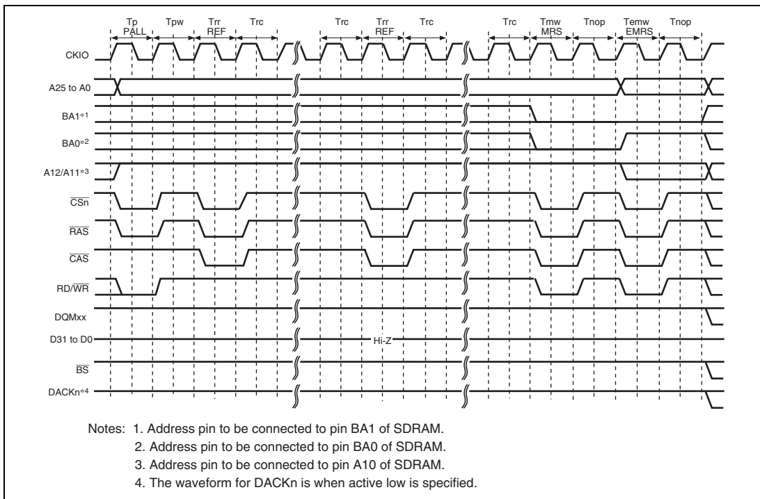
Figure 10.31 EMRS Command Issue Timing
