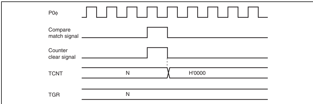
Figure 12.84 Counter Clear Timing (Compare Match)
