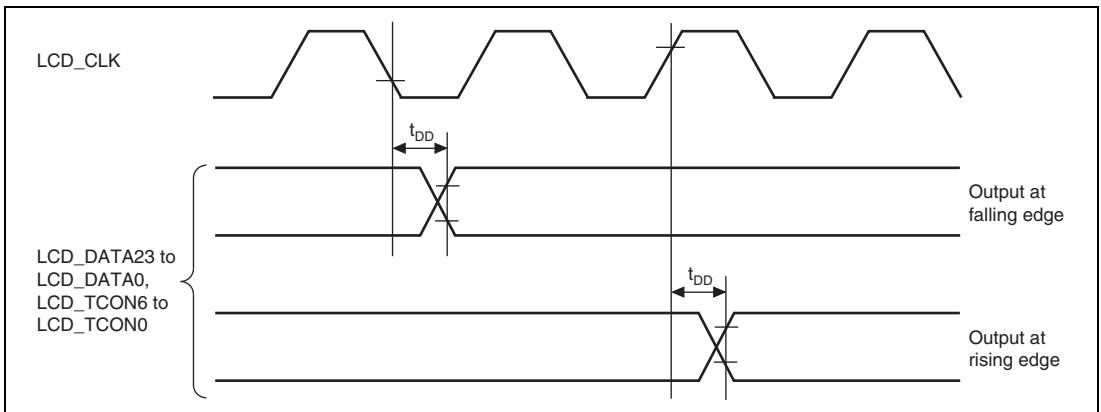
Figure 52.80 Display Output Timing
