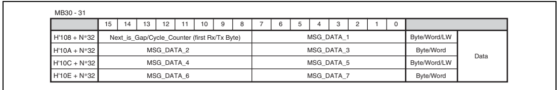
Figure 23.5 Message Data Field
