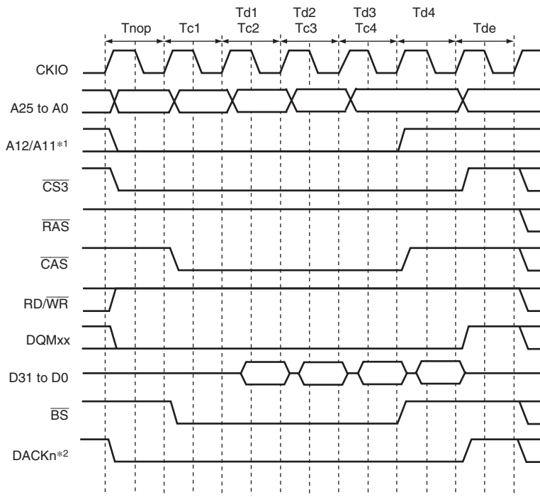
Figure 10.22 Burst Read Timing (Bank Active, Same Row Addresses in the Same Bank, CAS Latency 1)
