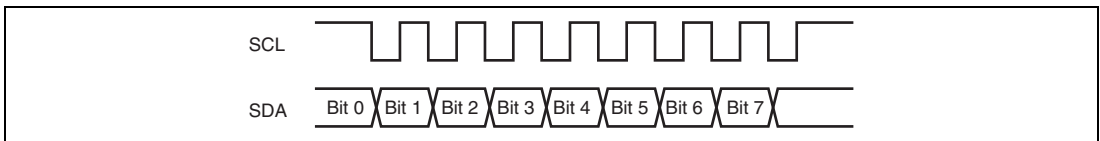
Figure 20.13 Clocked Synchronous Serial Transfer Format
