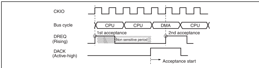
Figure 11.11 Example of DREQ Input Detection in Cycle Steal Mode Edge Detection
