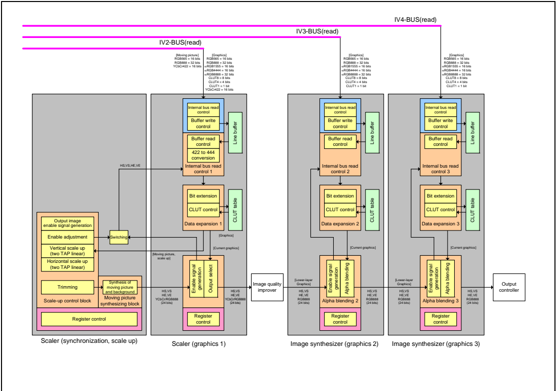
Figure 35.1 Functional Block Diagram of Image Synthesizer
