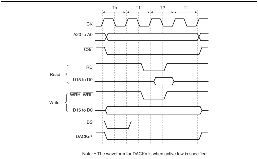
Figure 9.9 \overline{\text{CSn}} Assert Period Expansion
