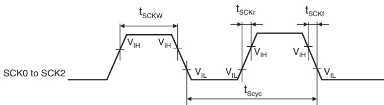
Figure 29.22 Input Clock Timing
