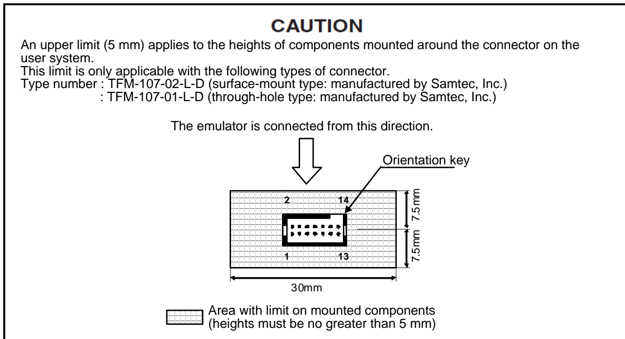
Figure 3 Limit on Height of Components Mounted around the Connector on the User System (the Connector for the Adapter)
