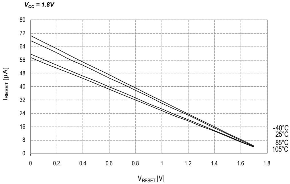
Figure 33-137. Reset Pin Pull-up Resistor Current vs. Reset Pin Voltage
