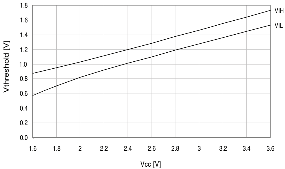
Figure 33-274. I/O Pin Input Threshold Voltage vs. V_{CC} T = 25^\circ\text{C}
