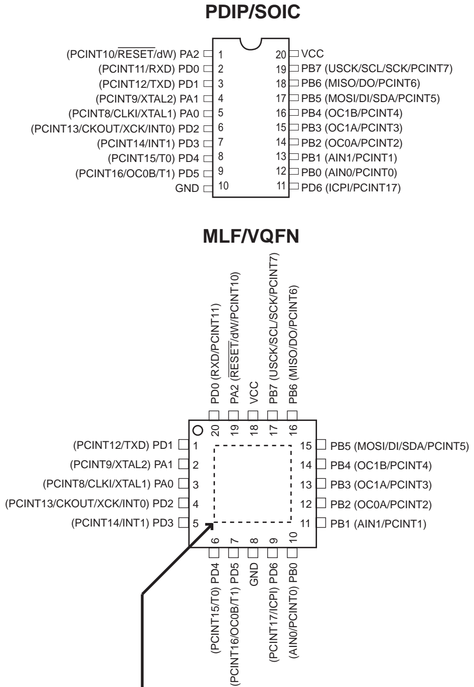
Figure 1-1. Pinout ATtiny2313A/4313
