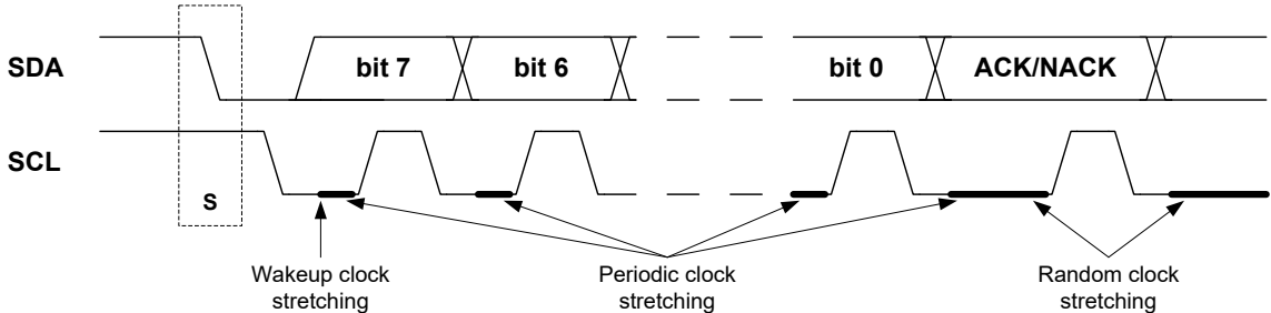
Figure 25-9. Clock Stretching (1)
