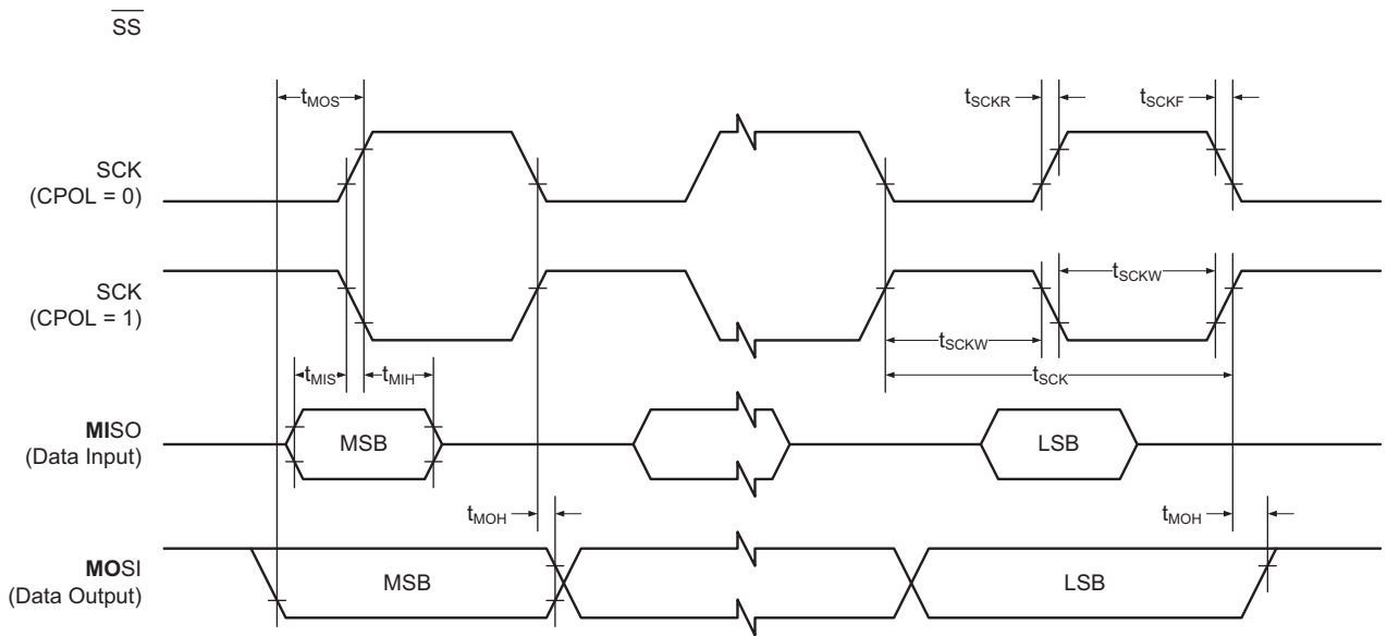
Figure 32-19. SPI Timing Requirements in Master Mode
