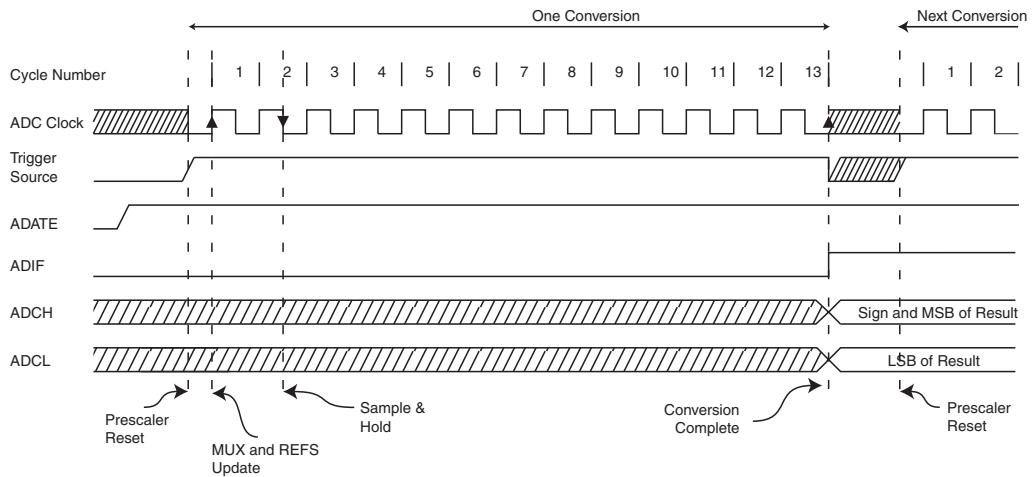
Figure 24-6. ADC Timing Diagram, Auto Triggerged Conversion
