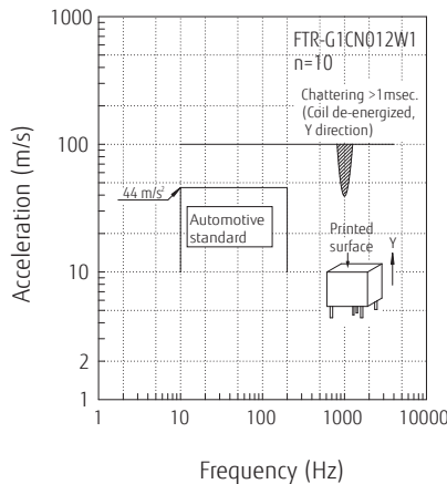
Vibration resistance
