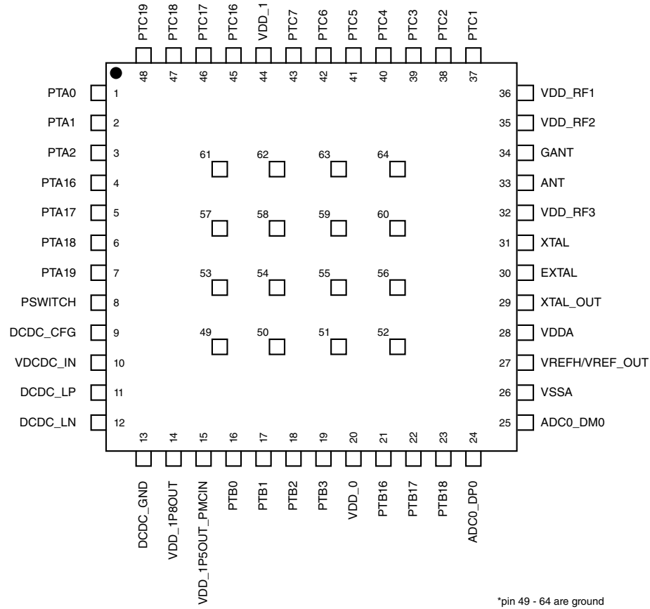
Figure 19. 48-pin Laminated QFN pinout diagram
