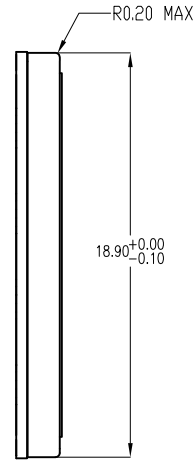
SIDE VIEW - RF INPUTS
