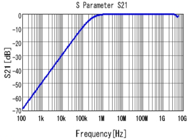
■ GRM188R71H562KA01 S21 DCOV, 25degC
