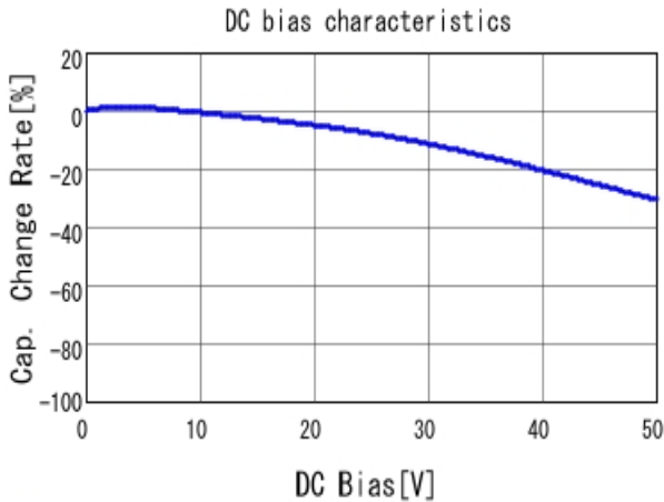
■ GRM188R71H562KA01 C-DC bias capchange, 25.0degC, AC1.
