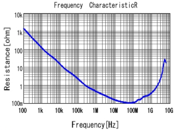
■ GRM188R71H562KA01 R DCOV, 25degC
