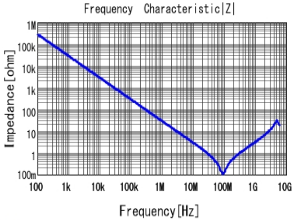
■ GRM188R71H562KA01 |Z| DCOV, 25degC
