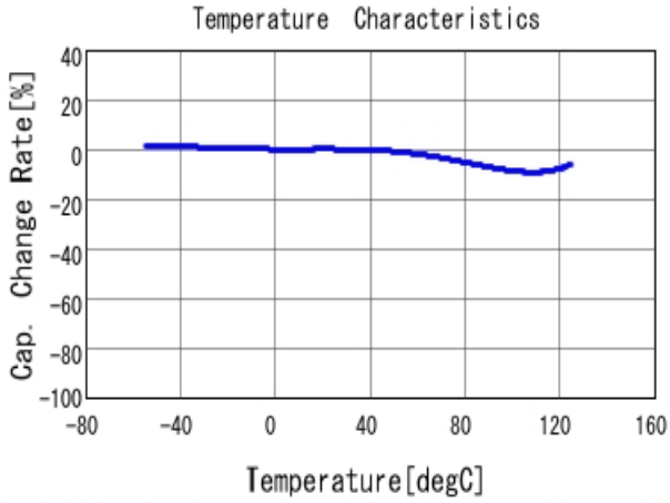
■ GRM188R71H562KA01 C-Temp. capchange, DCO. 0V, AC1.0V rm
