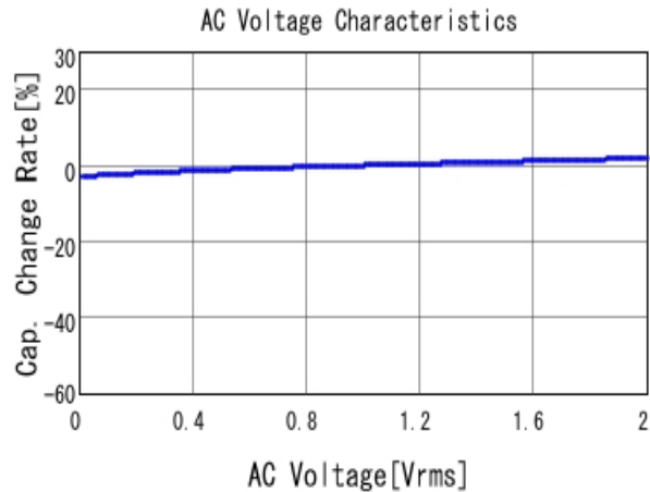
■ GRM188R71H562KA01 C-AC Voltage capchange, DCOV, 25.0d
