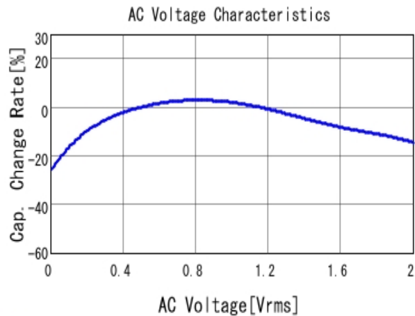
■ GRM188R60G226MEA0 C-AC Voltage capchange, DCOV, 25.0d
