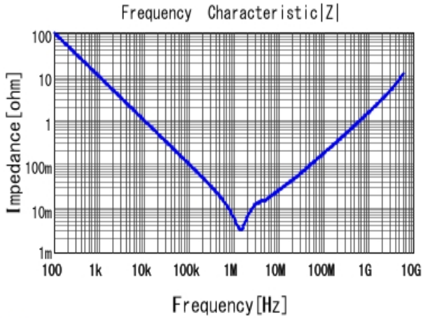
■ GRM188R60G226MEA0 |Z| DCOV, 25degC
