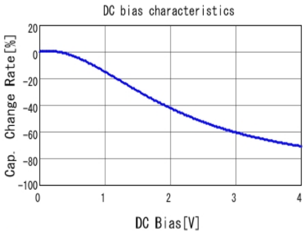
■ GRM188R60G226MEA0 C-DC bias capchange, 25.0degC, AC0.
