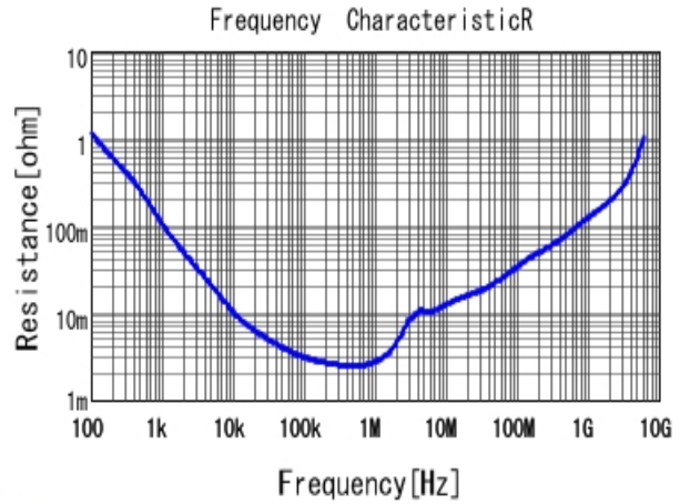
■ GRM188R60G226MEA0 R DCOV, 25degC
