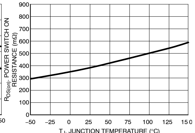
Figure 15. Power Switch R_{DS(on)} vs. Junction Temperature
