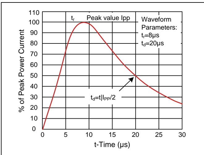
Figure 1. Pulse Waveforms
