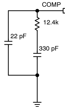
Figure 29. Recommended Compensation for Primary Switcher
