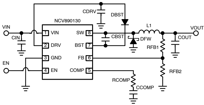
Figure 1. Typical Application
