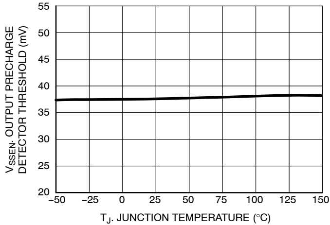
Figure 24. Output Precharge Detector Threshold vs. Junction Temperature
