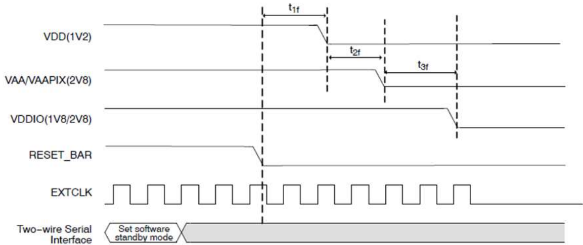
Figure 23. Power Down Sequence
