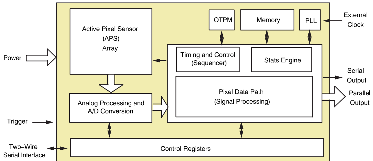
Figure 1. Block Diagram
