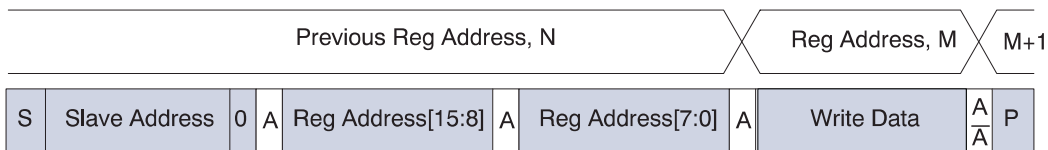
Figure 14. Single WRITE to Random Location
