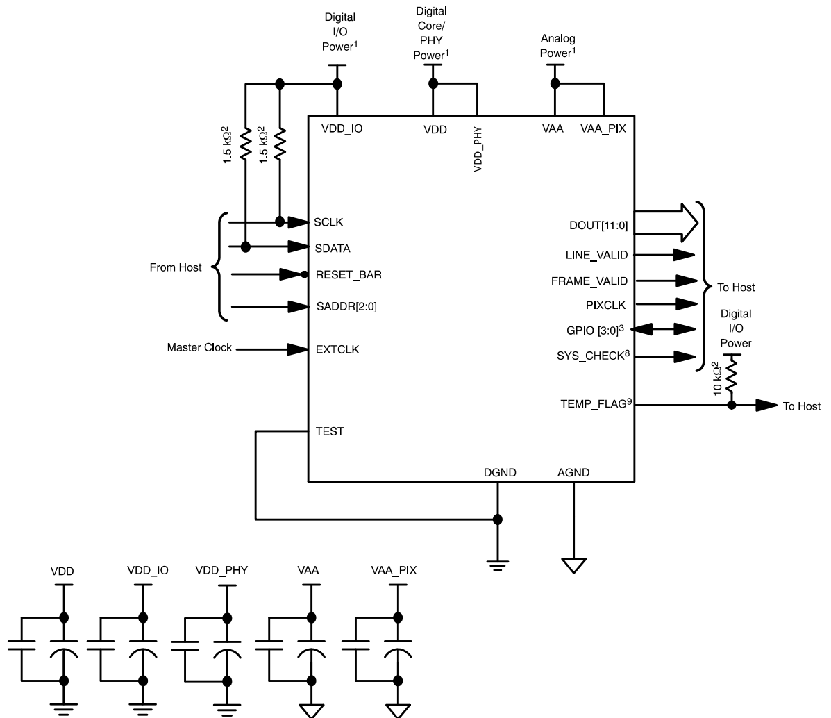
Figure 6. Typical Configuration, Parallel
