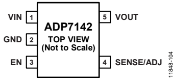
Figure 4. 5-Lead TSOT Pin Configuration
