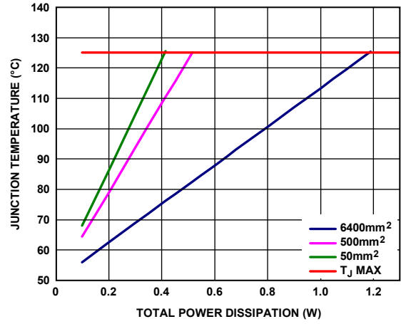
Figure 56. SOIC, T A = 50°C
