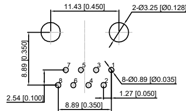
RECOMMENDED PCB LAYOUT VIEWED FROM COMPONENT SIDE
