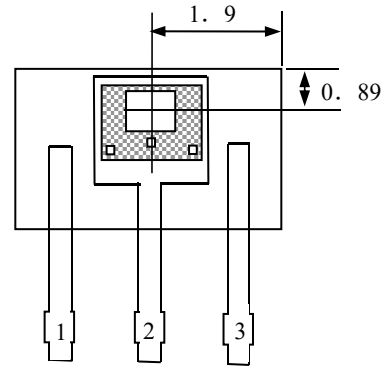
Sensor
