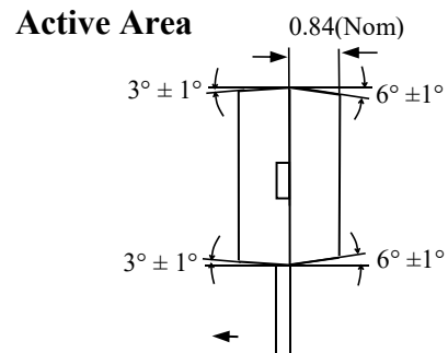
Sensor
