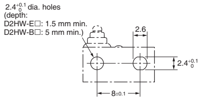
Mounting Hole Dimensions (Reference)
