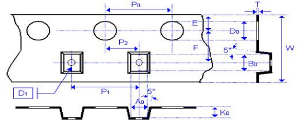
Fig. 9.2 The dimension of plastic tape
