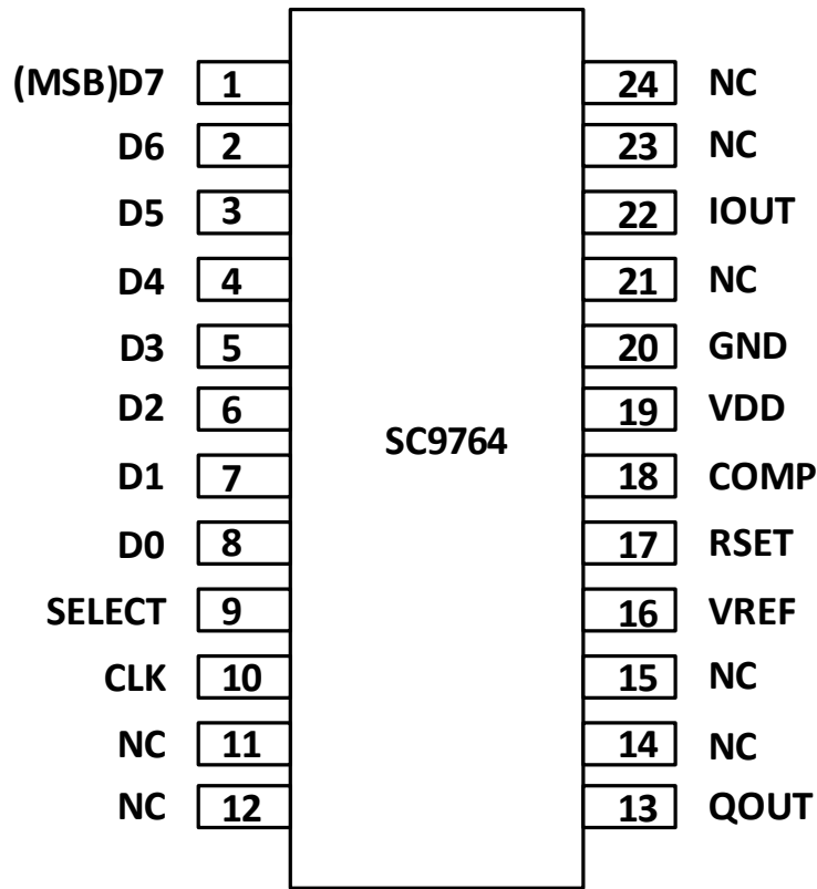
Figure2. Pin Configuration
