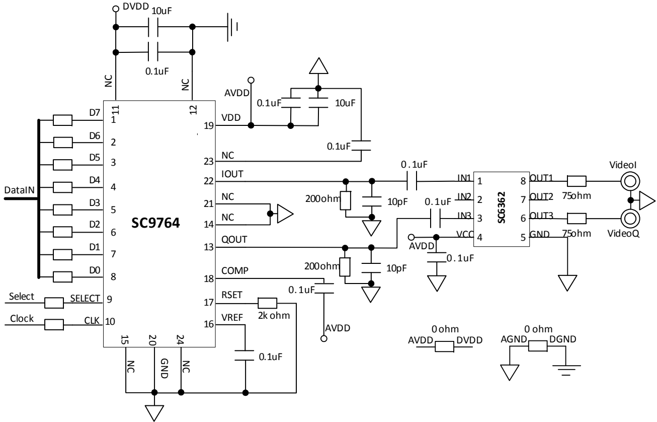
Figure 4. Application Schematic for compatible with SC9766
