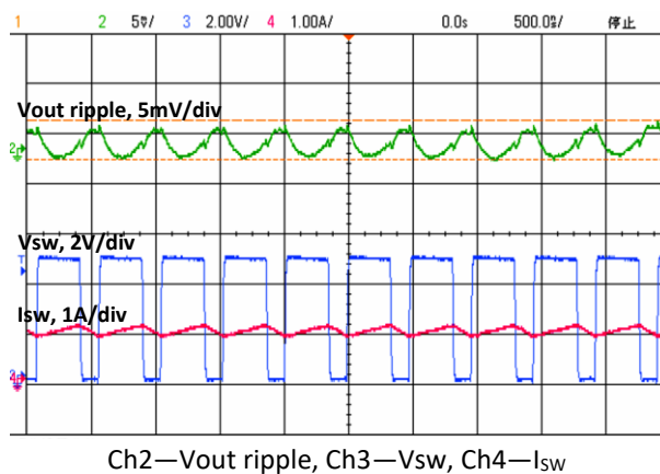
Output Ripple and SW at 1A load Vin=5V / Vout=3.3V
