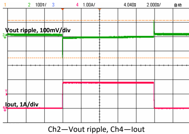
Vin=5V / Vout=1.8V / Iout=0.01~1.8A
