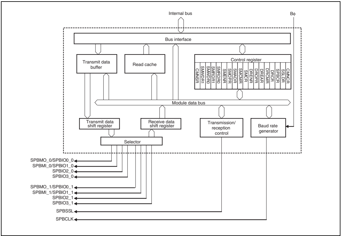
Figure 18.1 Block Diagram
