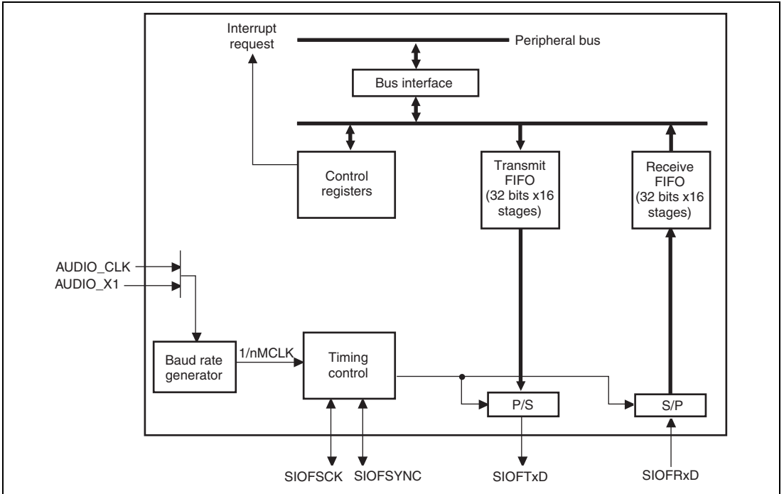
Figure 21.1 Block Diagram
