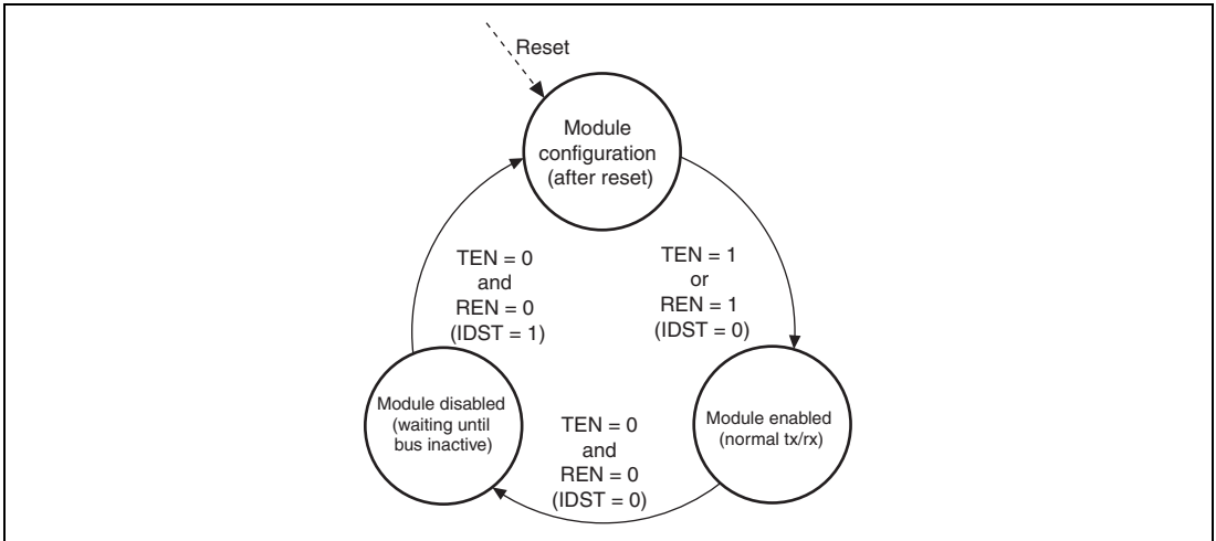
Figure 20.22 Operation Modes
