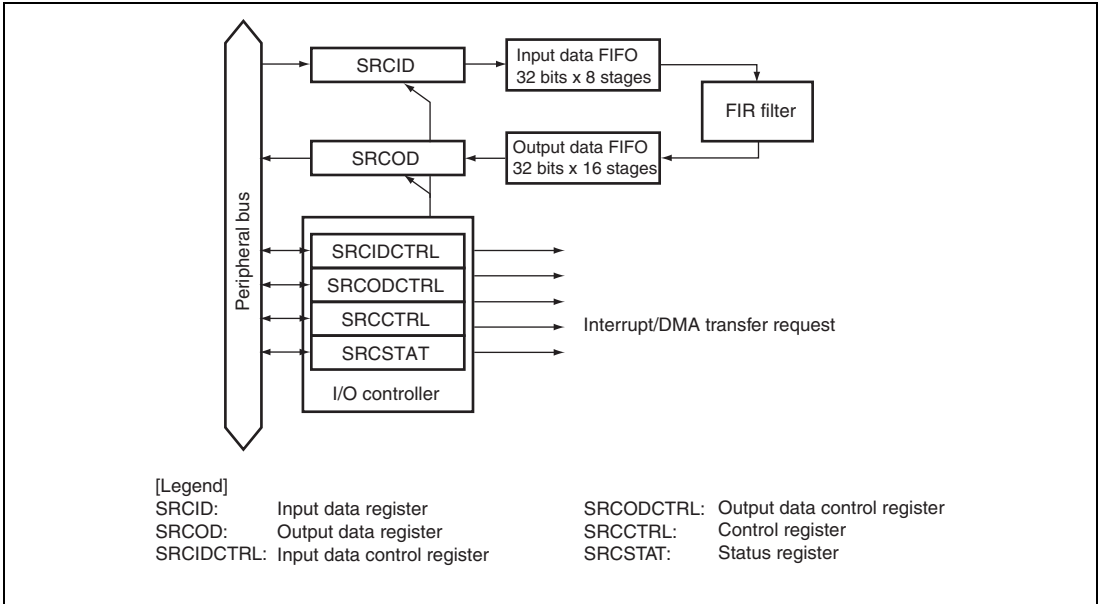
Figure 28.1 Block Diagram
