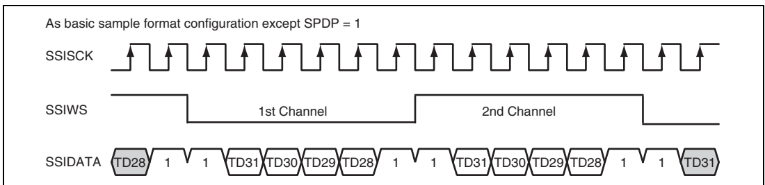
Figure 20.12 Inverted Padding Polarity
