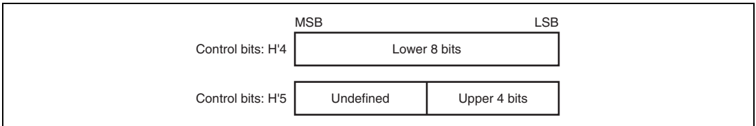
Figure 23.3 Locked Address Configuration
