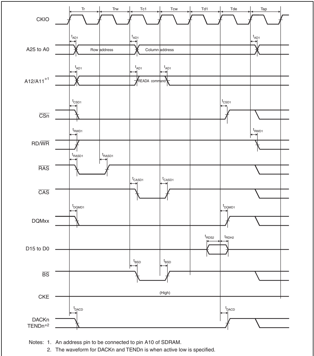
Figure 35.16 Synchronous DRAM Single Read Bus Cycle (Auto Precharge, CAS Latency 2, WTRCD = 1 Cycle, WTRP = 1 Cycle)
