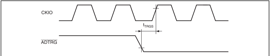
Figure 35.56 A/D Converter External Trigger Input Timing
