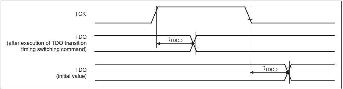
Figure 33.3 User Debugging Interface Data Transfer Timing
