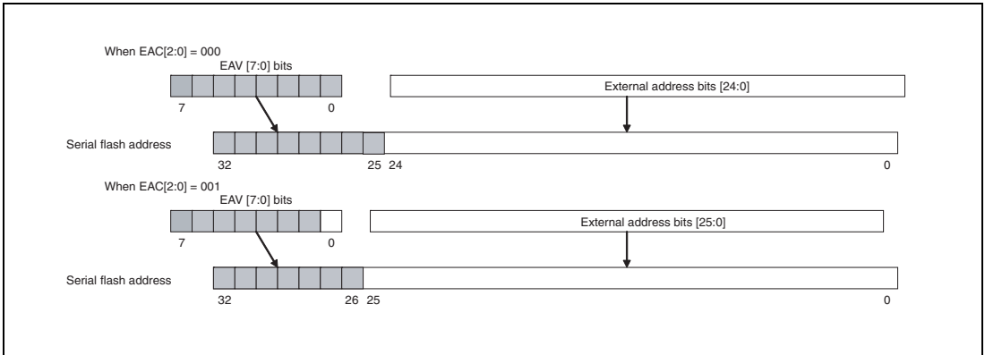
Figure 18.4 32-Bit Address Setting
