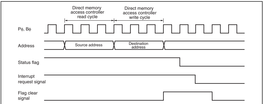
Figure 12.97 Timing for Status Flag Clearing by Direct Memory Access Controller Activation
