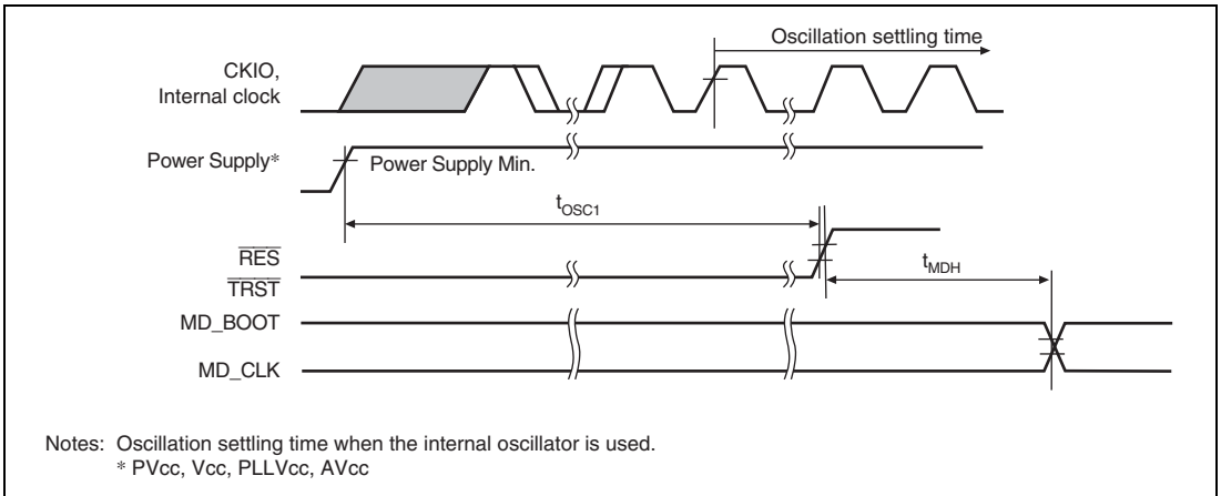
Figure 35.3 Power-On Oscillation Settling Time
