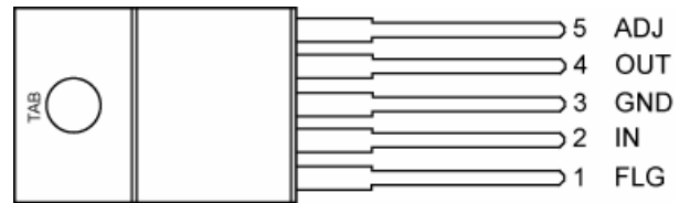
5-Pin TO-220 Adjustable with Flag (T) LM29153/29303/29503
