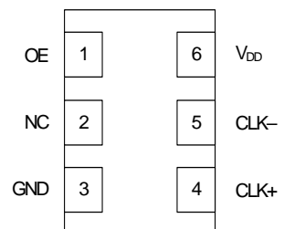
Si591 (LVDS/LVPECL/CML)
