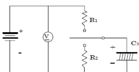
Fig. 9 Surge voltage circuit
