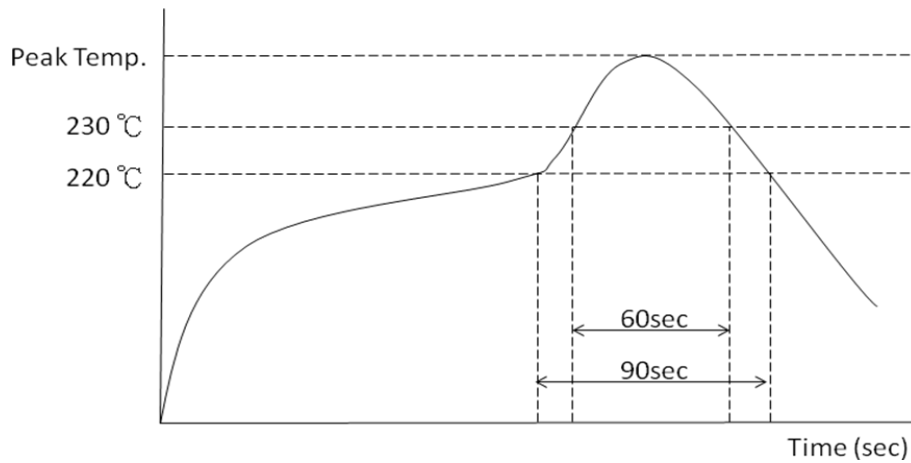
Figure 4 Reflow profile
