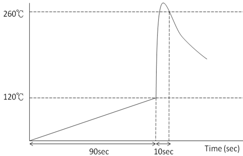
Figure 6 Flow Curve
