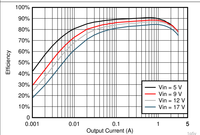
Figure 7-11. V_{OUT} = 1.5 V Efficiency, L = 1.5 \mu\text{H}
