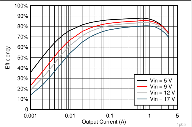
Figure 7-10. V_{OUT} = 1.05 V Efficiency, L = 1.2 \mu\text{H}
