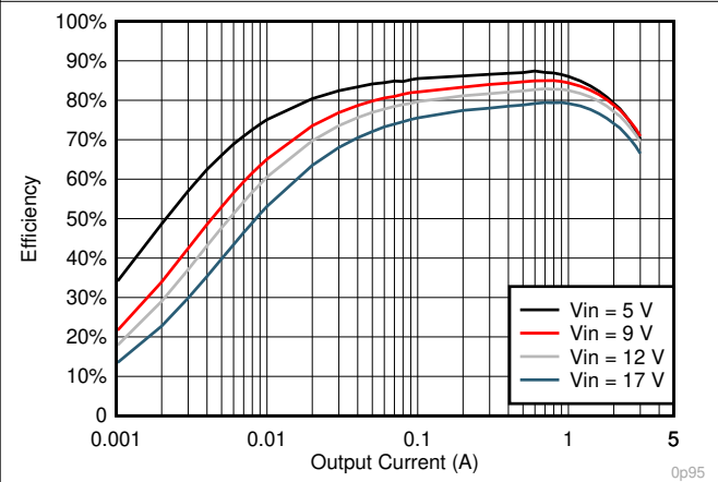
Figure 7-9. V_{OUT} = 0.95 V Efficiency, L = 1.2 \mu\text{H}
