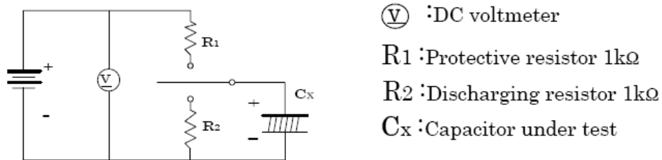
Fig. 4 Surge voltage circuit
