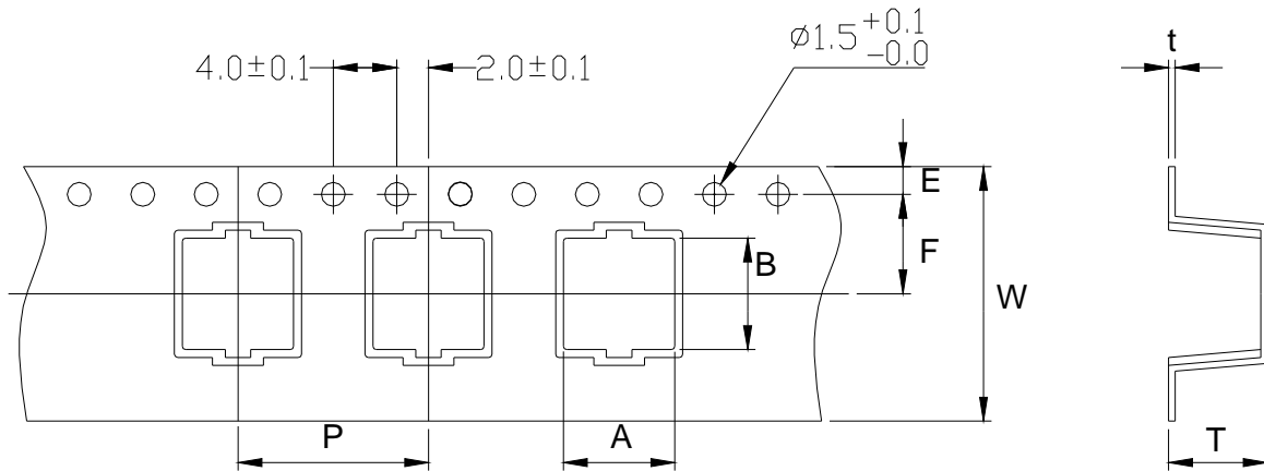
Fig. 6 Carrier tape
