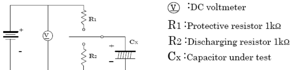
Fig. 9 Surge voltage circuit
