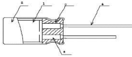
Fig. 1 Cross-section view
