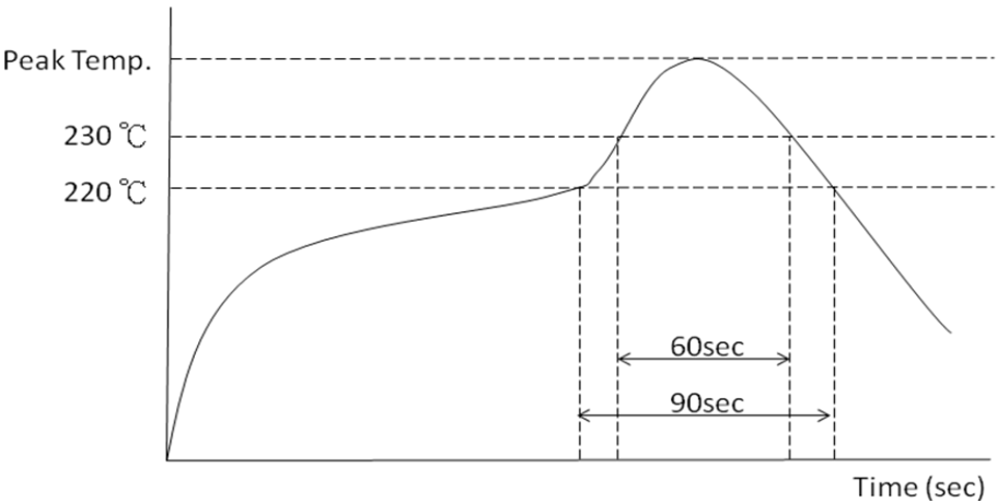
Figure 4 Reflow profile
