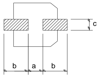
Figure 5 Soldering pad
